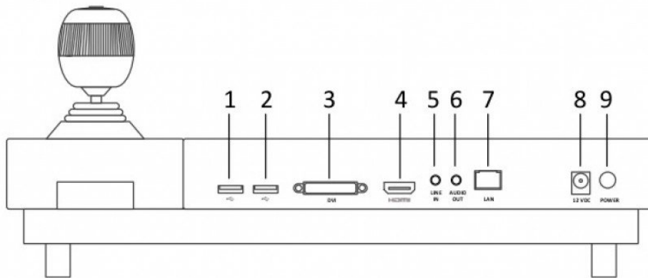
Figure 1.2 Rear Panel of DS-1600KI
